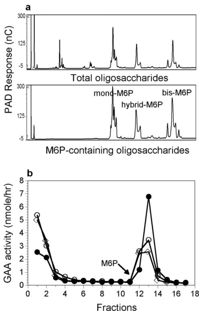
FIG. 2. a, analysis of the oligosaccharides released following digestion of \alpha -galactosidase A with endoglycosidase H (upper panel) and following purification of the M6P-containing fraction over a QAE column (lower panel) by Dionex column chromatography. b, chromatography of rhGAA (open circles), neo-rhGAA (closed circles), and periodate-treated rhGAA (open squares) over a CI-MPR column as described in the legend for Fig. 1. PAD, pulsed amperometric detection.
