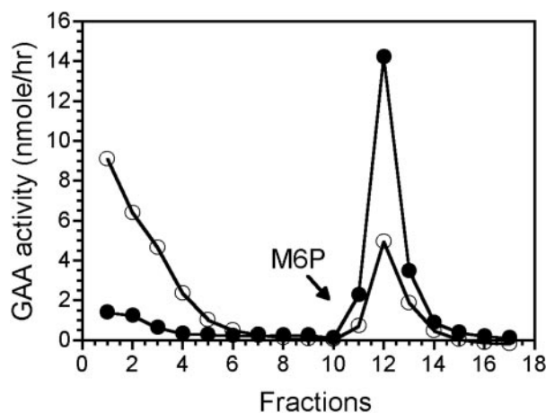
FIG. 1. Chromatography of rhGAA (open circles) and phosphopentamannose-conjugated rhGAA (closed circles) over a CI-MPR column. Approximately 10 \mu g of each of the enzymes was loaded onto a 2-ml CI-MPR column. After washing the column with binding buffer, the bound material was eluted (starting at fraction 11) with binding buffer containing 5 mM M6P. Two-ml fractions were collected and assayed for GAA activity.
